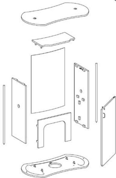
SPO5 exploded view
