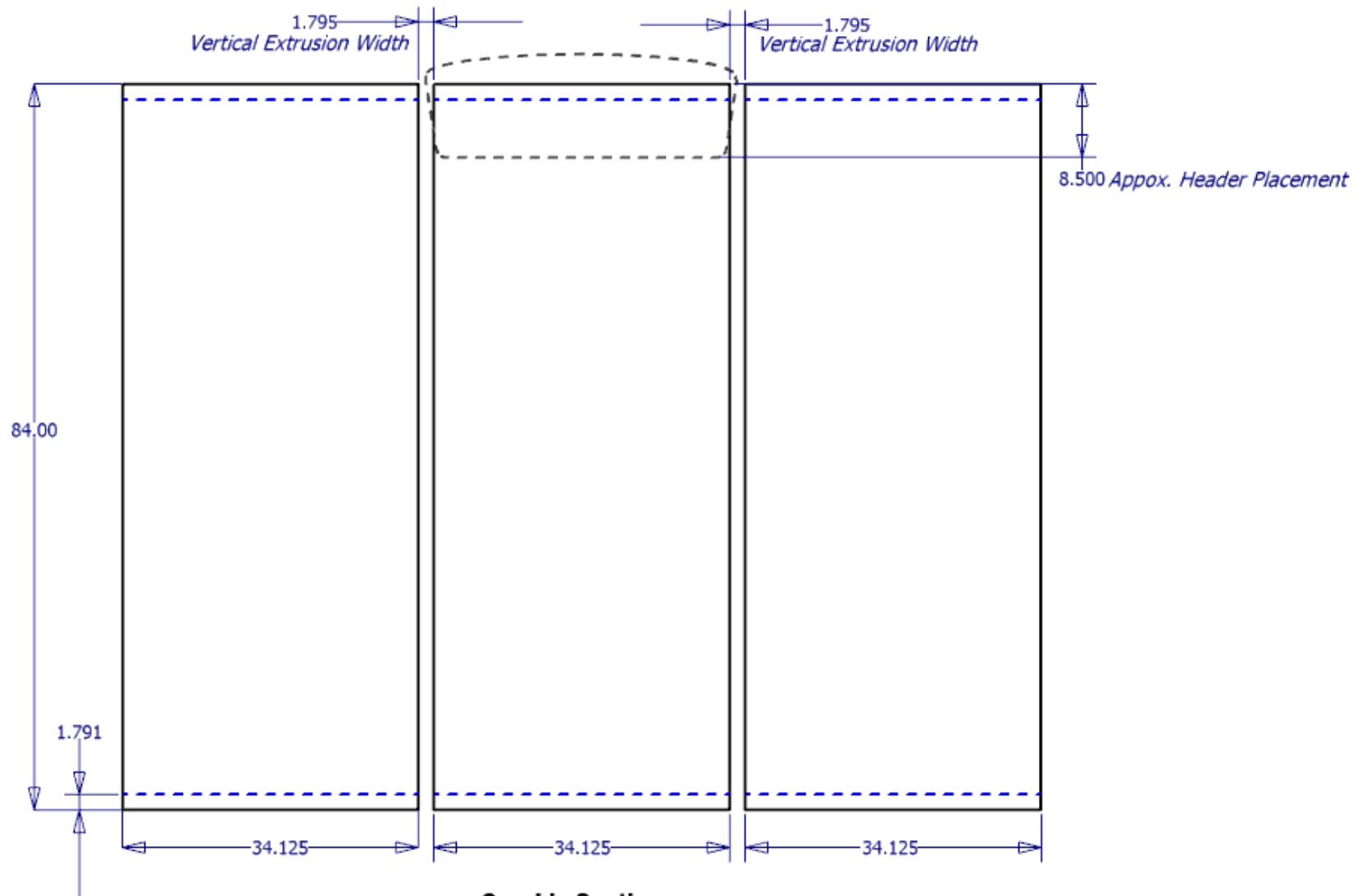
Graphic Section (Dash equals Extrusion Height)
